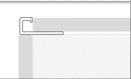
Chiusura perimetrale a muro/ Wall covering edging
