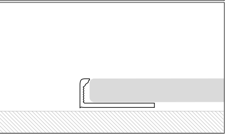
Chiusura perimetrale a muro/ Wall covering edging
